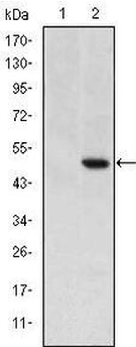
Cripto Antibody (MA5-15843) in WB Western blot analysis of TDGF1 using TDGF1 monoclonal antibody (Product # MA5-15843) in HEK293 (1) and TDGF1 (AA: 31-188) human IgG Fc transfected HEK293 (2) cell lysate.
