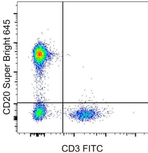
CD20 Antibody (64-0209-42) in Flow Staining of normal human peripheral blood cells with Anti-Human CD3 FITC (Product # 11-0038-42) and Anti-Human CD20 Super Bright 645. Cells in the lymphocyte gate were used for analysis.
