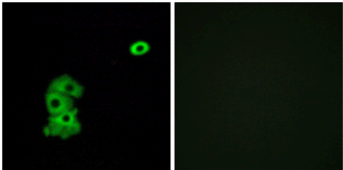
OR4C6 Antibody (PA5-38230) in ICC/IF Immunofluorescent analysis of OR4C6 in A549 cells using an OR4C6 polyclonal antibody (Product # PA5-38230).
