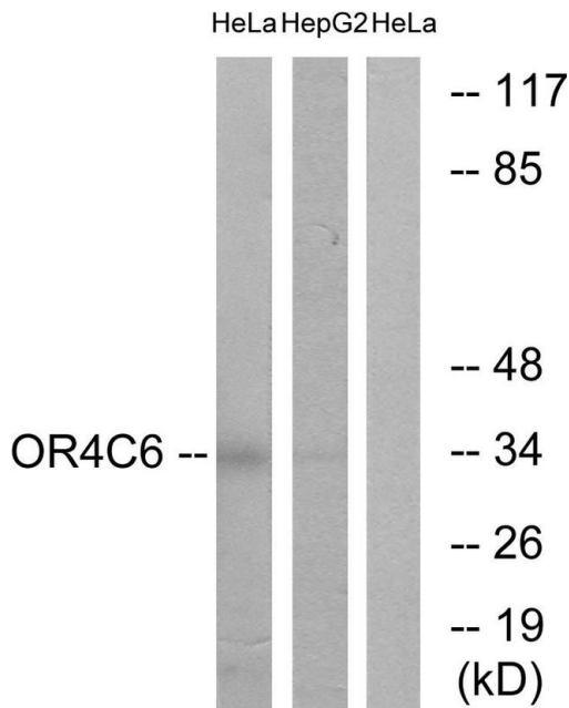
OR4C6 Antibody (PA5-38230) in WB Western blot analysis of OR4C6 in extracts from HeLa cells and HepG2 cells using an OR4C6 polyclonal antibody (Product # PA5-38230).
