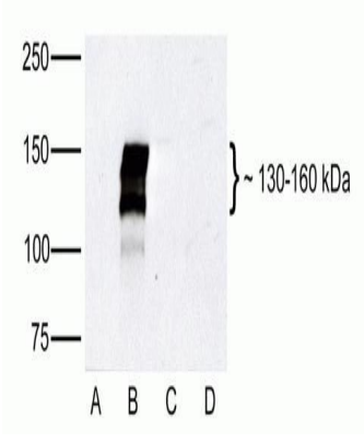
ZO-2 Antibody (38-9000) in WB Western blot analysis of human Caco-2 cells (lane B) using Zymed (R) Rb anti-ZO-2 (Mid) (Product # 38-9000). Antibody does not react with dog (MDCK cell lysates, lane A), rat (KNRK cell lysates, lane C), or mouse (TCMK-1 cell lysates, lane D).
